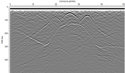
2. F:\DATA\MIGRATION_TOPO\PROC\DATA\M_F_00001EY.151 / traces: 252 / samples: 416
